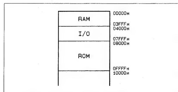
Fig. 5-4-1. Address Map (SY-69 Board)
